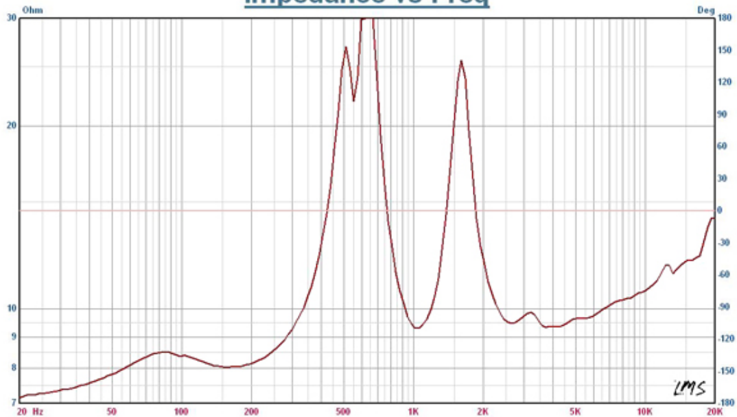
Impedance vs Freq
